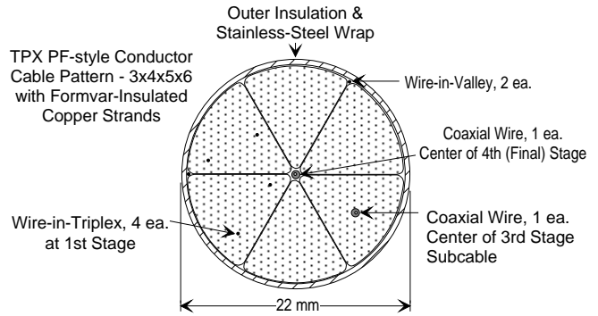
Figure 2: Cable Configuration for the NRTC
