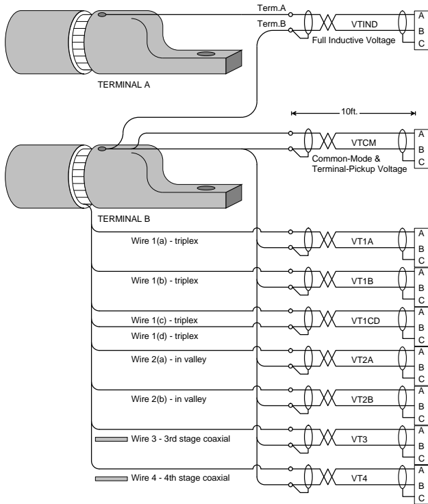
Figure 5: Sensor Wiring Diagram for the NRTC
