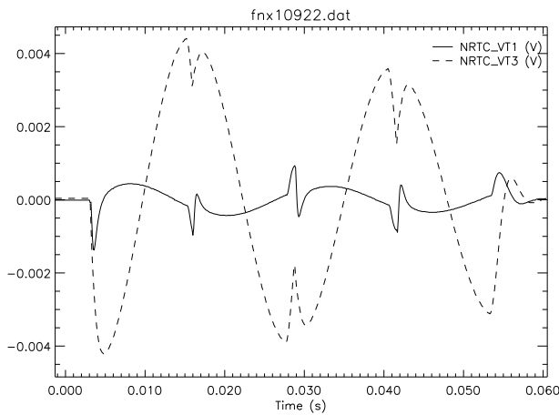
Figure 8: 2-Coil Transverse-Field NRE Data
