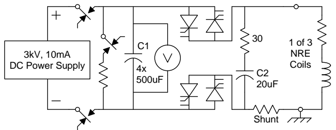
Figure 4: JAERI Power Supply for the NRE
