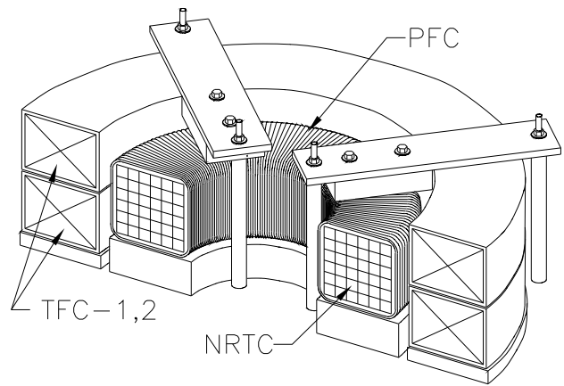
Figure 3: Coil Configuration for the NRE
