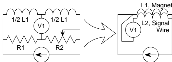
Figure 1: Balanced-Bridge & Co-Wound Sensor Quench Detection
